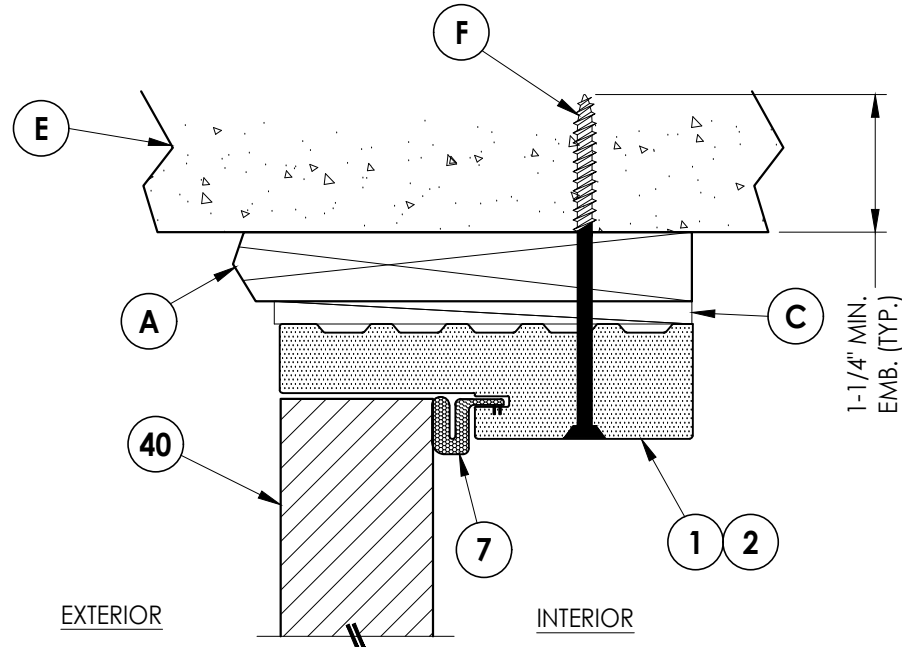
4 9 VERTICAL CROSS SECTION Outswing Shown (Inswing Similar) Shown w/ 1X Buck
