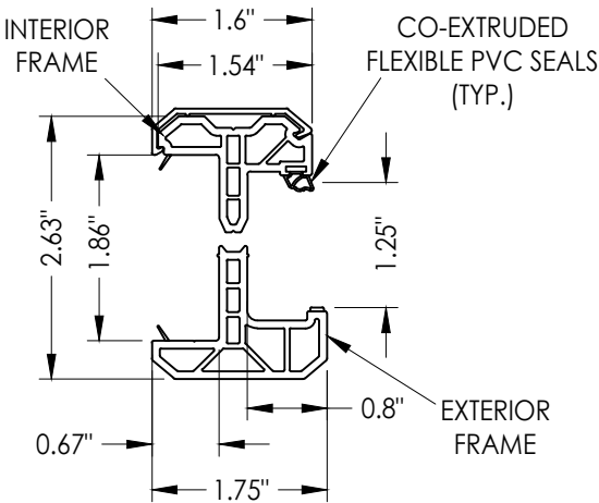
5B ODL KEYSTONE PVC LITE FRAME 1-1/4" GLAZING
