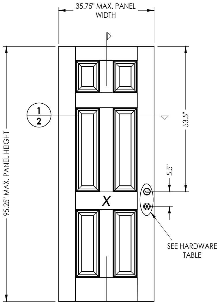
2 2 FIBERGLASS DOOR PANEL ODL
