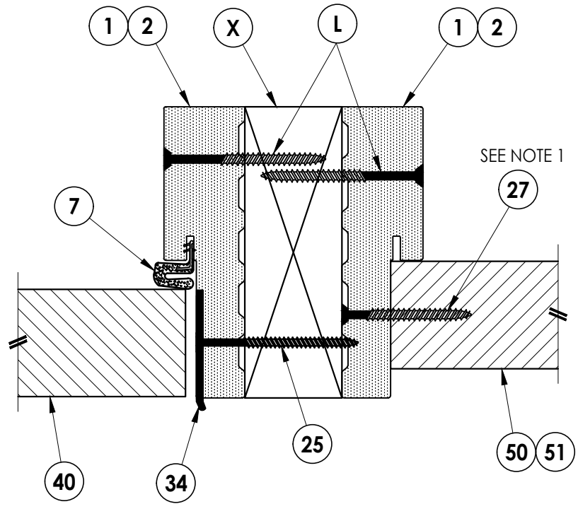
2 7 HORIZONTAL CROSS SECTION Outswing Shown (Inswing Similar)
