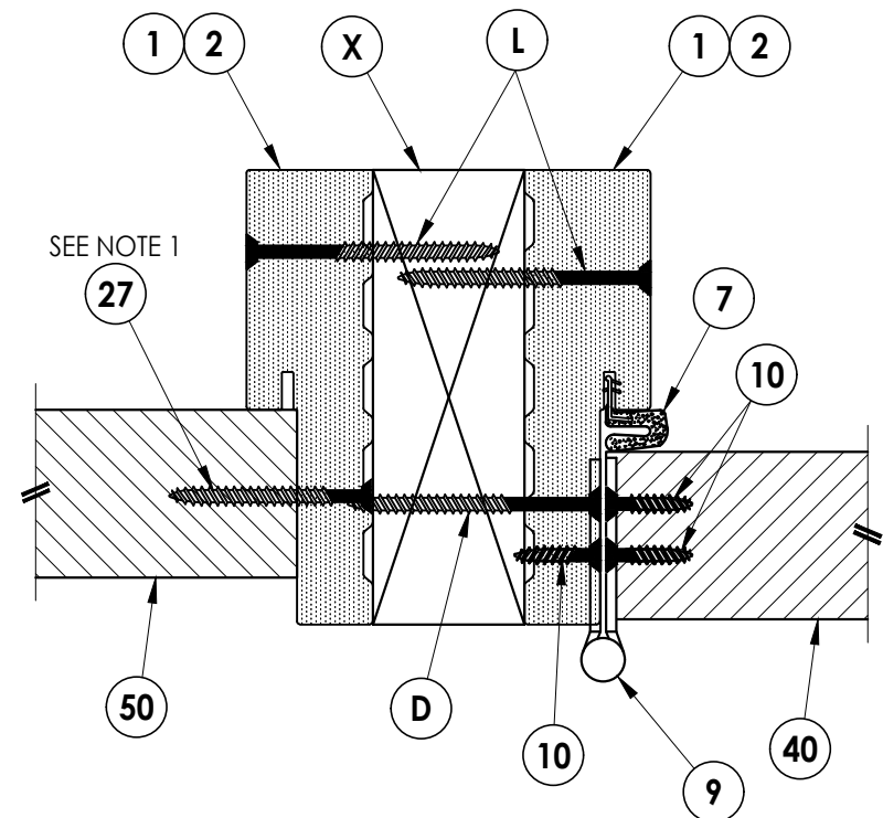
1 7 HORIZONTAL CROSS SECTION Outswing Shown (Inswing Similar)
